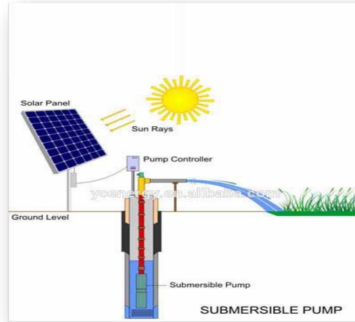
Solar Submersible Pump
